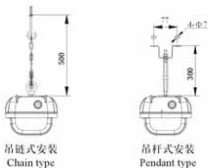
全塑三防荧光灯 Full plastic weather-proof fluorescent light fittings
