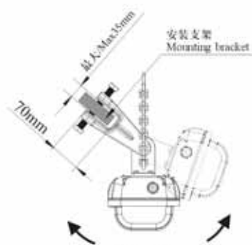
角度可调 The angle is adjustable
