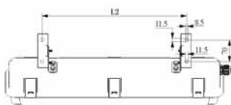
可调支架安装 Adjustable mounting bracket
